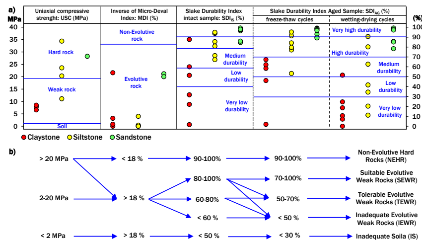
fig 3. a) Geomechanical results of studied samples. b) Weak rock classification for use in road embankments.
