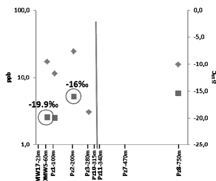
fig. 2. TCE isotopic signature (δ 13 C) (squares) obtained from the different wells installed along the plume and in distance from the focus. The vertical line corresponds to the place where the ZVI-PRB is installed. The diamonds indicate the concentration of TCE in each point.
